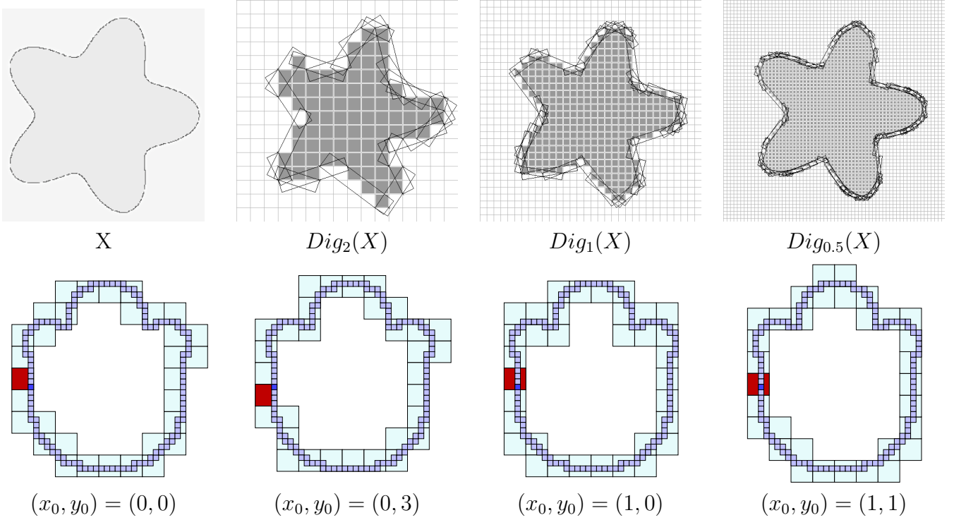
Figure 1: First row: Illustration of the digitization process Dig_h(\cdot) applied on the real shape X with the set of maximal segments covering the digital contours. Second row: Illustration of several subsampling with the same digitization grid size but with different shifts (x_0, y_0) .
