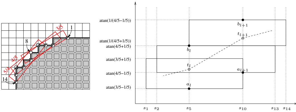
Fig. 4. Estimation of the possible tangent directions of shapes that are digitized as the black pixels. On the left, the maximal segments surrounding point C_8 are displayed with their slope. Each one defines possible tangent directions for their included points. It is enough to consider points that are extremities of a maximal segment to define a piecewise linear tangent representation of a contour which stays within the boxes. The bounds a and b are displayed for two of these points on the right.
