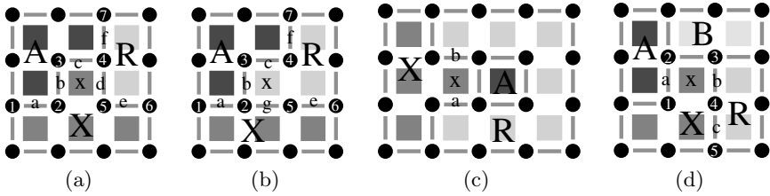
Fig. 2. Examples of ML-simple points and non ML-simple points. (a) x is ML-simple for R . c(x, R) = (\{\}, \{d\}) and c(x, X) = (\{\}, \{g\}) are homotopic to 1-disks. c^-(x, A) = (\{2, 3, 4\}, \{b, c\}) is simple for f(X, A) = (\{1, 2, 3, 4\}, \{a, b, c\}) ; and add-simple for f(R, A) = (\{4, 7\}, \{f\}) . (b) Partition obtained from (a) after the flip of x in R . f(X, R) = (\{2, 5, 6\}, \{e, g\}) , f(X, A) = (\{1, 2\}, \{a\}) , f(R, A) = (\{2, 3, 4, 7\}, \{b, c, f\}) . (c) x is not a ML-simple point for R because c(x, R) = (\{\}, \{a, b\}) is not homotopic to a 1-disk. Flipping x in R modifies the topology of R . (d) x is not a ML-simple point for R because c^-(x, A) = (\{1, 2\}, \{a\}) is not add-simple for f(R, A) = (\{\}, \{\}) . Flipping x in R modifies the adjacency between regions.
